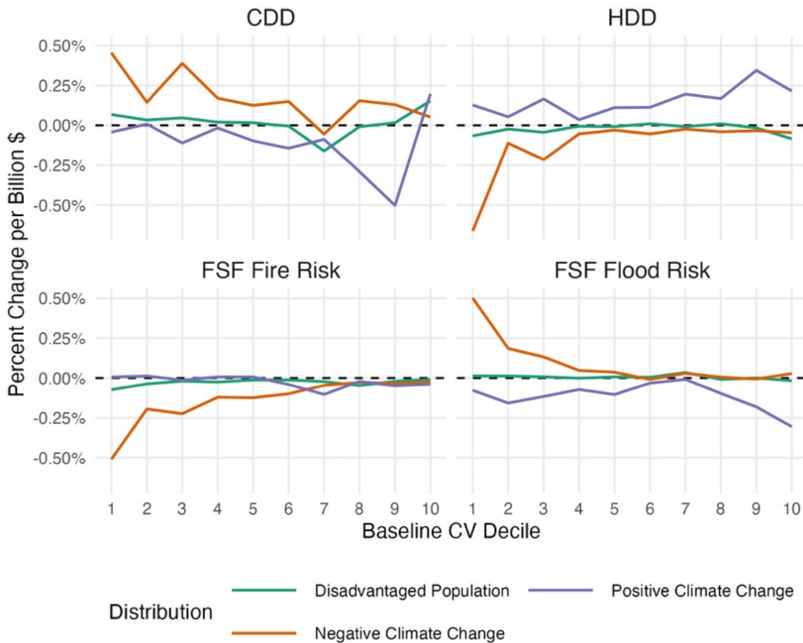
Figure 11: Change in climate with subsidies relative to without subsidies for households in the lowest income decile. The X-axis is a household's decile in CV from the baseline simulation comparing 2019 and 1990 climates relative to the entire population. We have filtered to just households below the 10th income percentile in the baseline simulation. We calculate the values on the Y-axis as a percent change in the respective climate variable relative to baseline values for each group, normalized by the total amount of subsidies dispersed. See description in the text on the subsidy distributions
